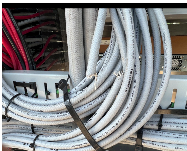
Left: Successful cuts and theft of wire in equipment cabinet. Top right: Cuts to wires on utility pole in conduit. Bottom right: Cuts to wires on utility pole in cabinet.
